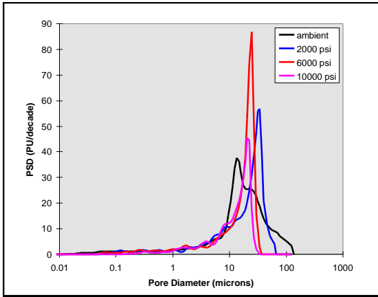
Figure 13 - Pore Size Distribution
