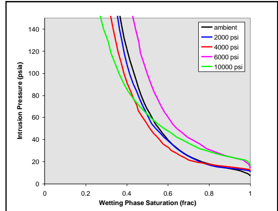
Figure 2 - Capillary Pressure Curves
