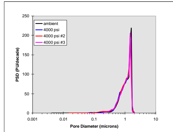
Figure 20 – Pore Size Distribution (4000 psi)
