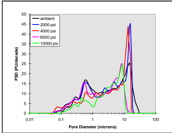
Figure 1 - Pore Size Distribution
