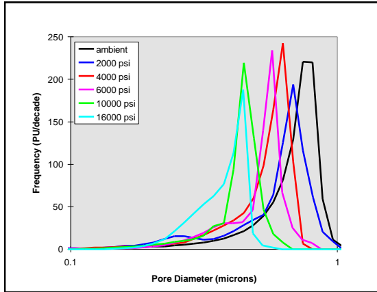
Figure 16 - Pore Size Distribution
