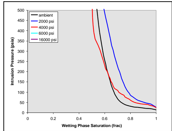
Figure 8 - Capillary Pressure Curves
