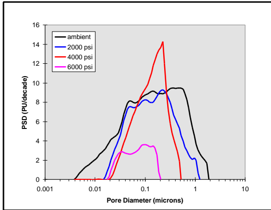
Figure 4 - Pore Size Distribution
