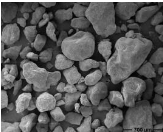
Figure 15 - SEM Micrograph
