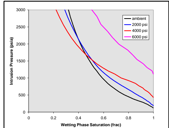
Figure 5 - Capillary Pressure Curves
