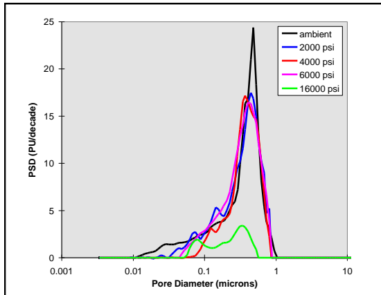
Figure 10 - Pore Size Distribution
