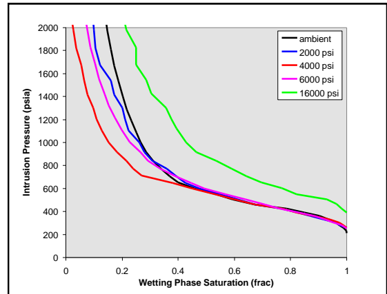
Figure 11 - Capillary Pressure Curves
