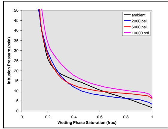
Figure 14 - Capillary Pressure Curves
