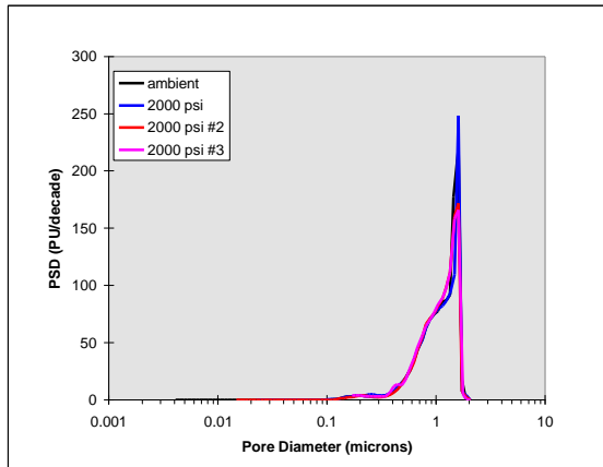
Figure 19 - Pore Size Distribution (2000 psi)
