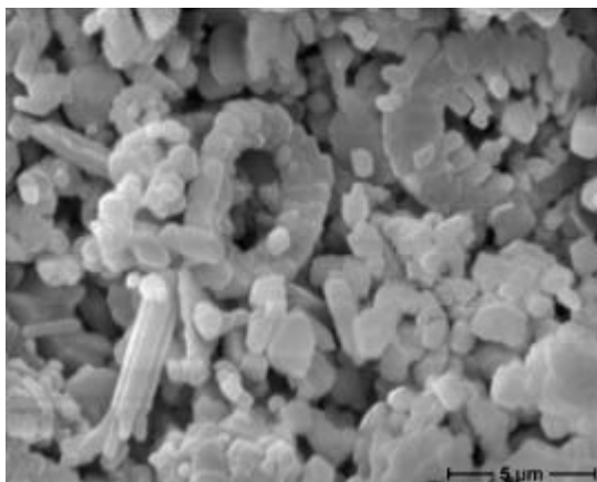
Figure 18 - SEM Micrograph
