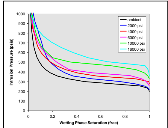
Figure 17 - Capillary Pressure Curves
